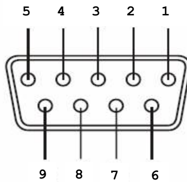
DB-9 Serial Connector
